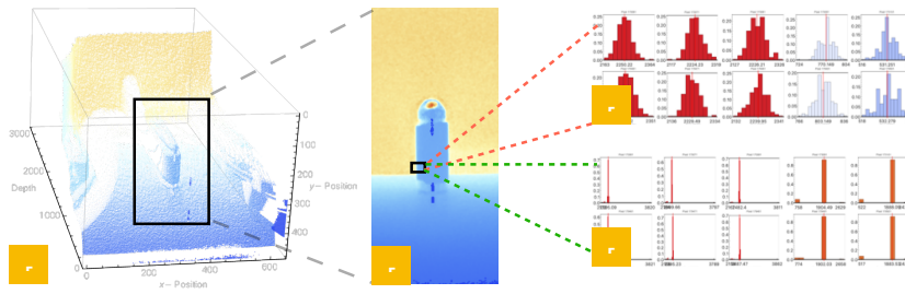
Figure 1. Figure 1. 3D depth image, [a], 2D view, [b], and quantified distance measurement uncertainty for two different distance-resolution modes of operation ([c], [d]), of a state-of-the-art LIDAR sensor. The uncertainty in individual locations of the depth measurement is not Gaussian, varies across pixels, and often has significant outliers (see [d])
